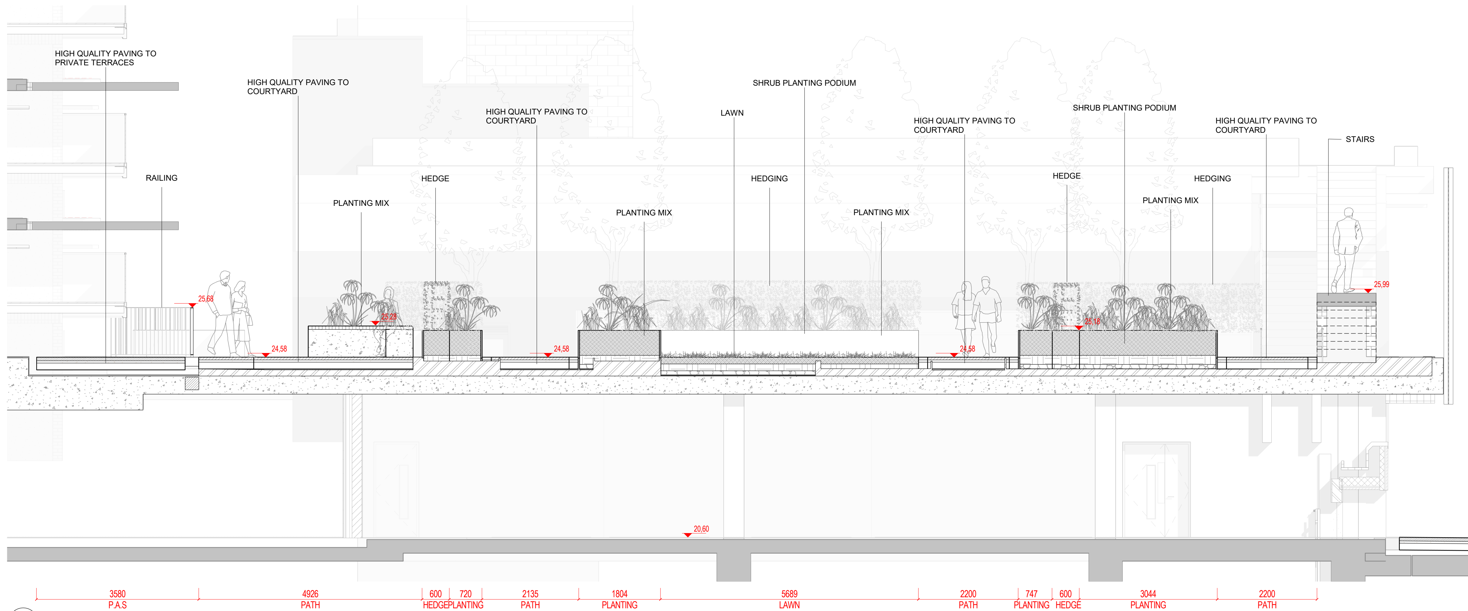
2 COURTYARD SECTION - BG2.4 1:50 @A1
